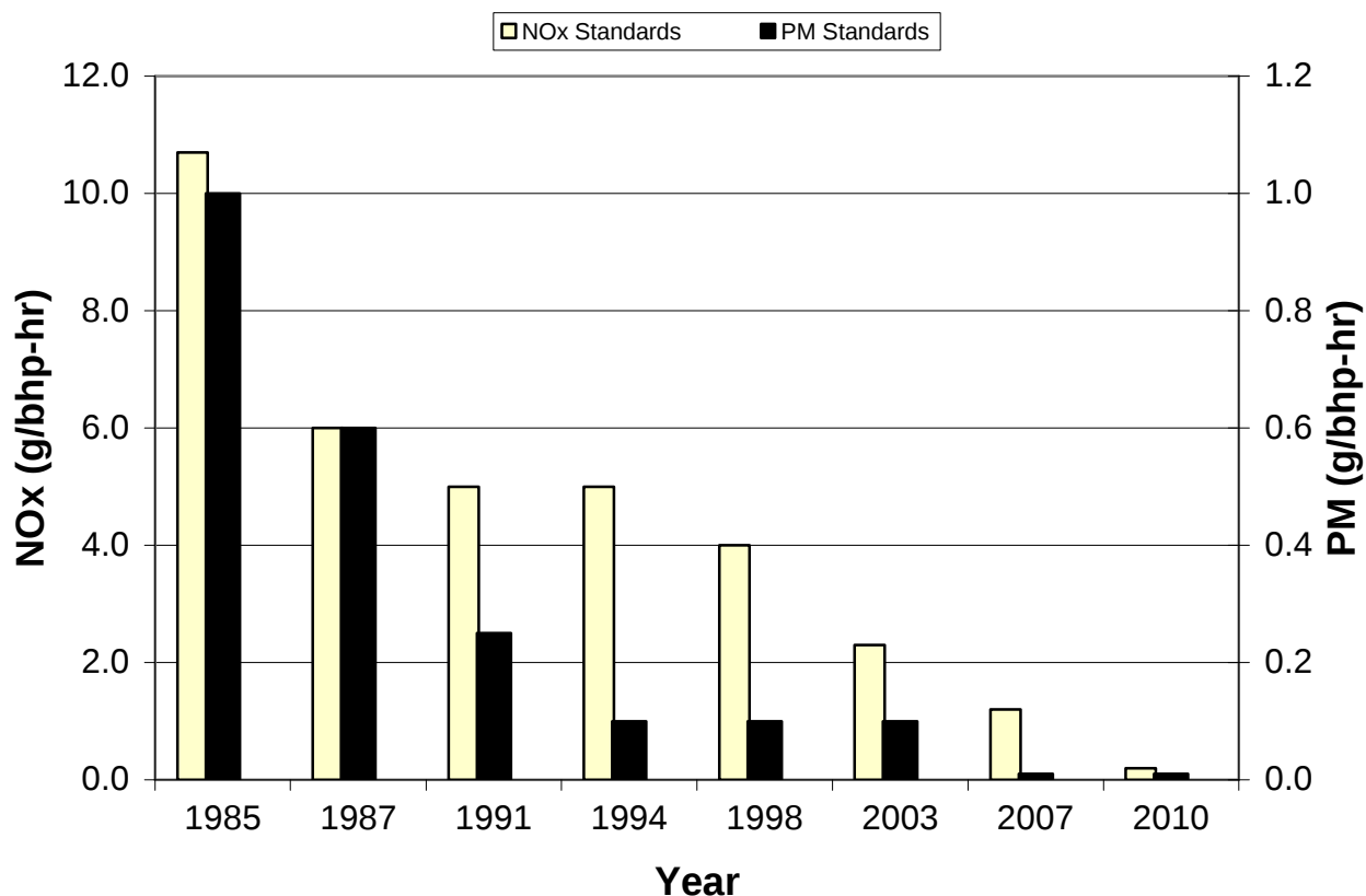
Figure II-6: California PM and NOx New Diesel Engine Emissions Standards (Based on Engine Model Year)
